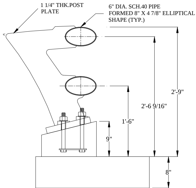
SBB40c - TXDOT T77 BRIDGE RAIL THUMBNAIL SKETCH
